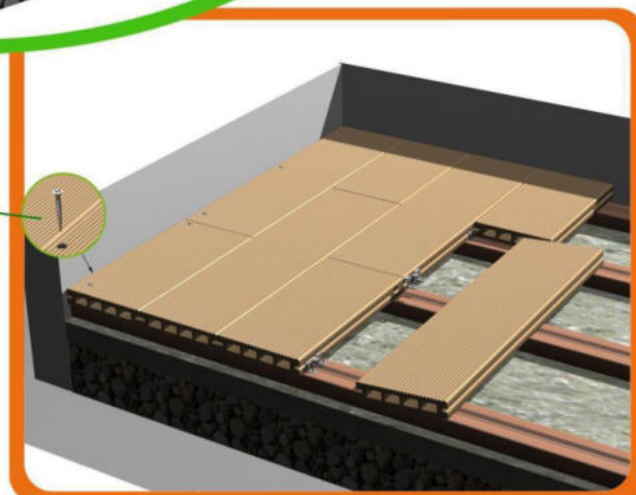
III、Insert decking/floor profiles into buckles/clips
